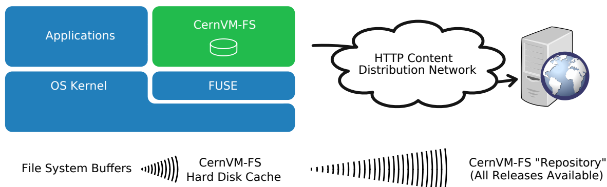
Fig. 1: A CernVM-FS client provides a virtual file system that loads data only on access. In this example, all releases of a software package (such as an HEP experiment framework) are hosted as a CernVM-FS repository on a web server.
